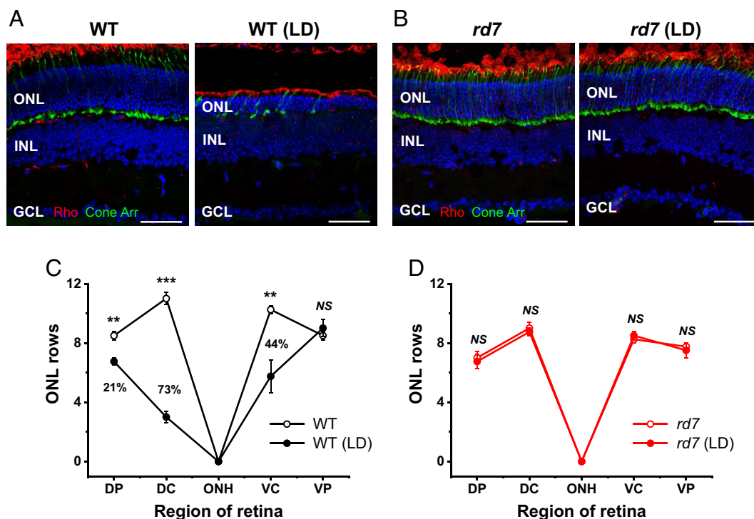
Fig. 1. Rods of rd7 mice are resistant to LD. ( A and B ) Cross-sections of dorsal-central retinas of WT ( A ) and rd7 ( B ) mice immunostained with anti-rhodopsin (red) and anti-cone arrestin (green) antibodies. Photoreceptor nuclei were counterstained with DAPI (blue). Four-month-old WT control ( A ) and rd7 ( B ) animals were either unexposed ( Left ) or exposed to bright white light (15 kLux) for 8 h ( Right ). ONL: outer nuclear layer, INL: inner nuclear layer, GCL: ganglion cell layer. (Scale bar, 50 \mu\text{m} .) ( C and D ) ONL thickness [quantified as the number of rows of photoreceptor nuclei (ONL rows)] in four regions of the retina from WT ( C ) and rd7 ( D ) animals either unexposed (open circles) or exposed to 15 kLux white light for 8 h (closed circles). DP: dorsal-peripheral, DC: dorsal-central, ONH: optic nerve head, VC: ventral-central, VP: ventral-peripheral. Values are means \pm SEM ( n = 4 in all cases). Statistical significances of the data are presented as **P < 0.01 , ***P < 0.001 , or NS (not significant, P > 0.05 ). Numbers show percentages of ONL thickness reduction in light-exposed mice compared to controls.
